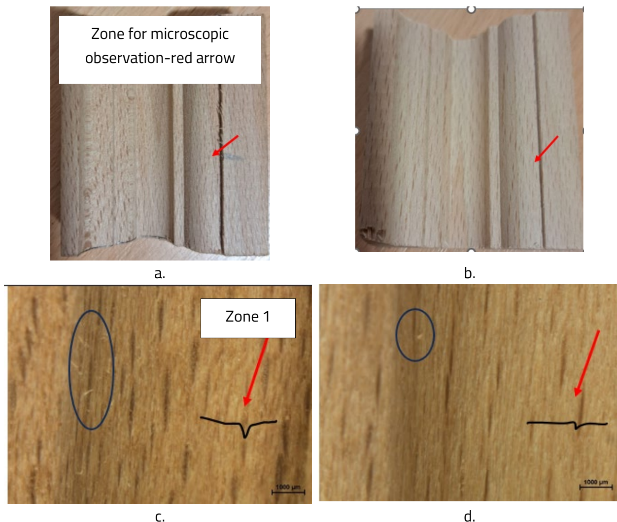
Fig. 59. Images of beech milled profiles (a, b) and microscopic details (c, d) at magnification 22.5x. (a, c) processing by n1-v_{f2} , sharpened tool; (b, d) processing by n1-v_{f2} -uzată, wear, tool after 600 m profile milling. Raised fibers are encircled with blue. (Brenci and Gurău 2024)
