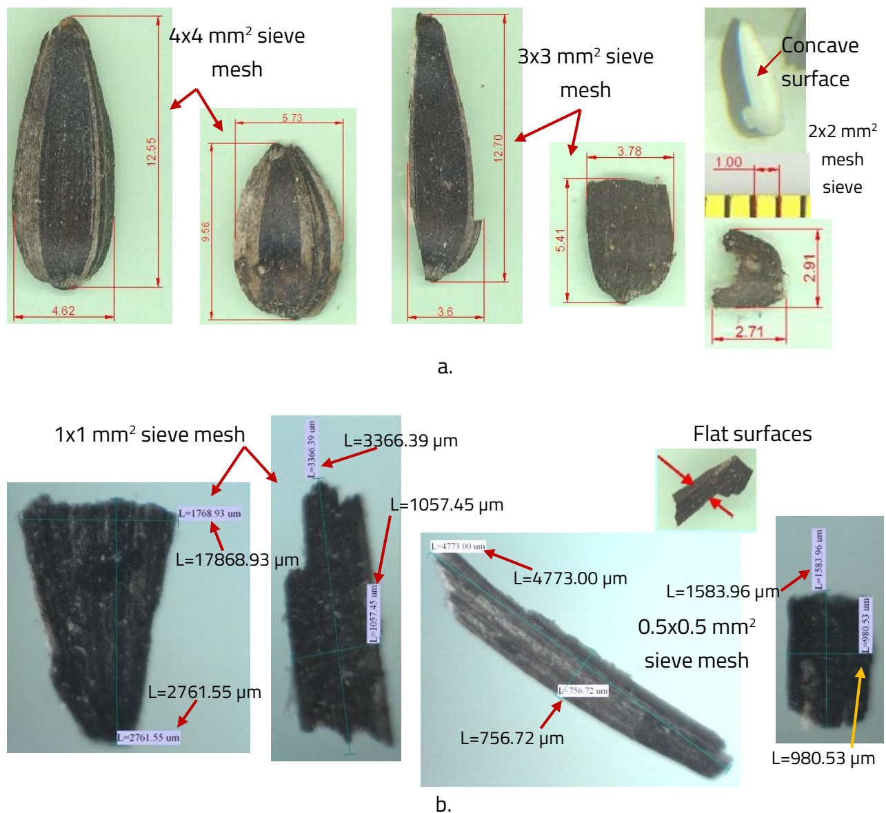
Fig. 3. Geometry and dimensions of sunflower seed husks (a) coarse particles; (b) fine particles (according to Coşereanu et al. 2015)
