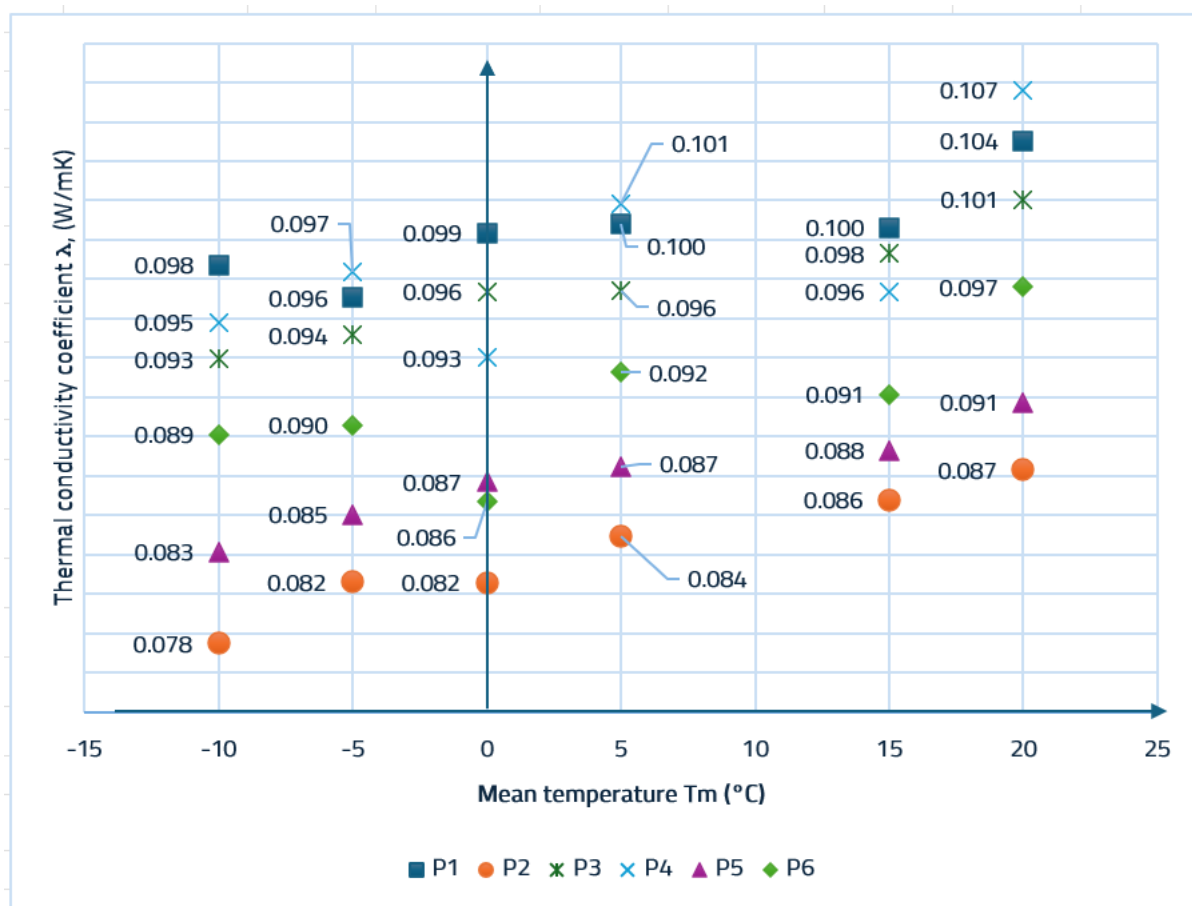
Fig. 30. Thermal conductivity coefficient of the panels manufactured (according to Brenci 2016)
