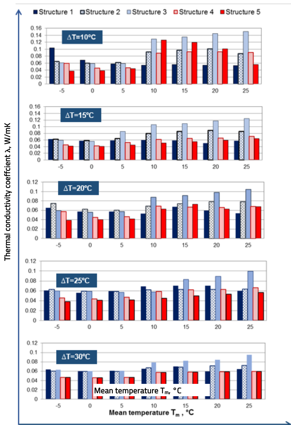
Fig. 21. Thermal conductivity coefficient values at various temperature differences between equipment hot plate and cold plate ( \Delta T ) and at different mean temperatures T_m (Brenci et al. 2018)
