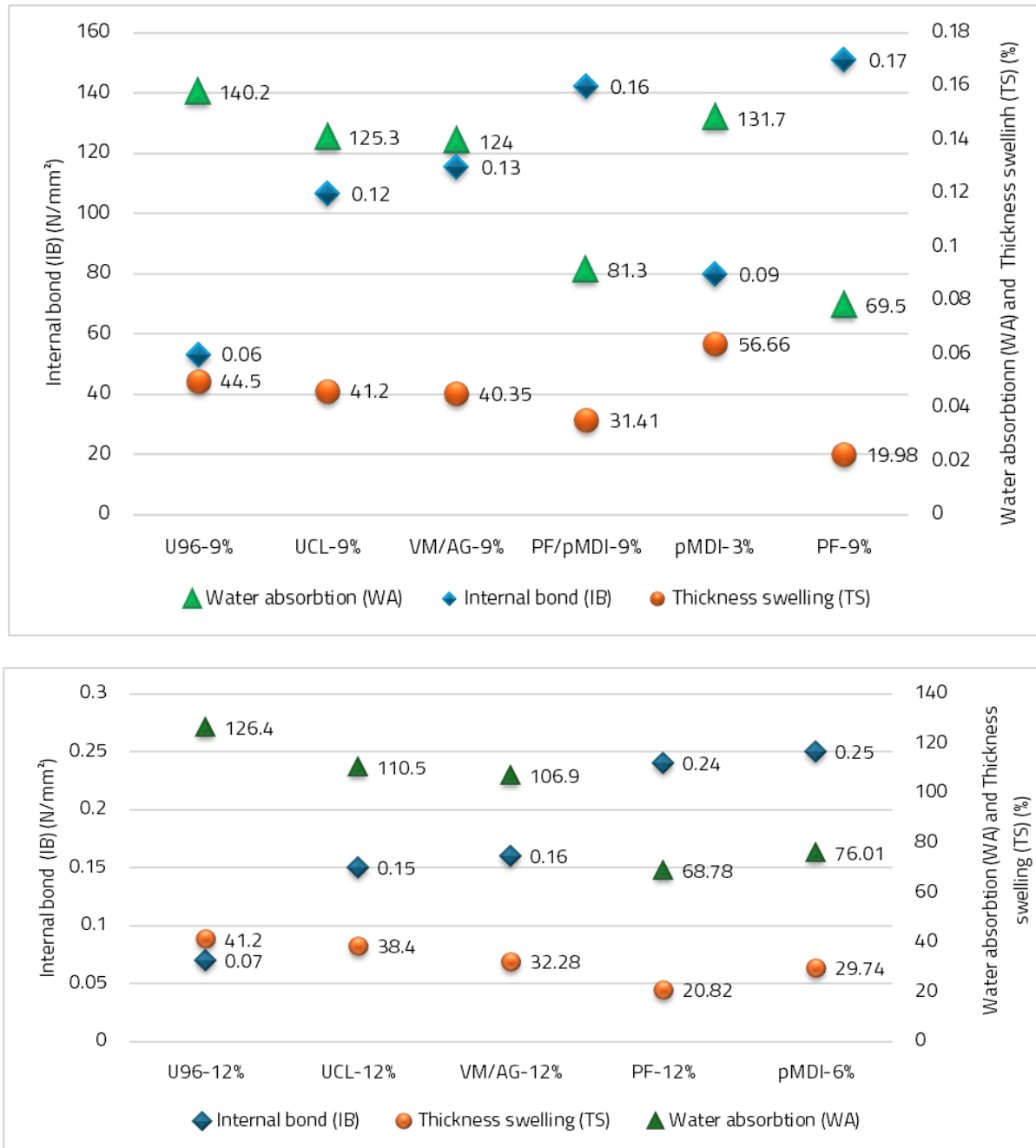
Fig. 18. Effect of adhesive type and content on thickness swelling (TS), water absorption (WA) and internal bond strength (IB) of modulus of elasticity (MOE) panels (according to Zeleniuc et al. 2019)
