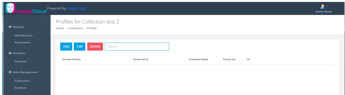
Fig. 42 Profile Interface
