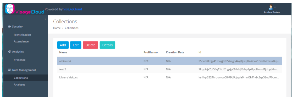
Fig. 41 Interfaces Collections
