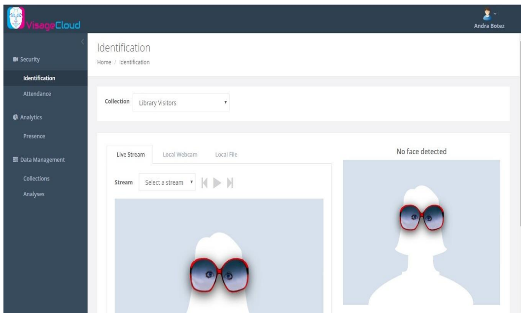
Fig. 44 Identifying users
