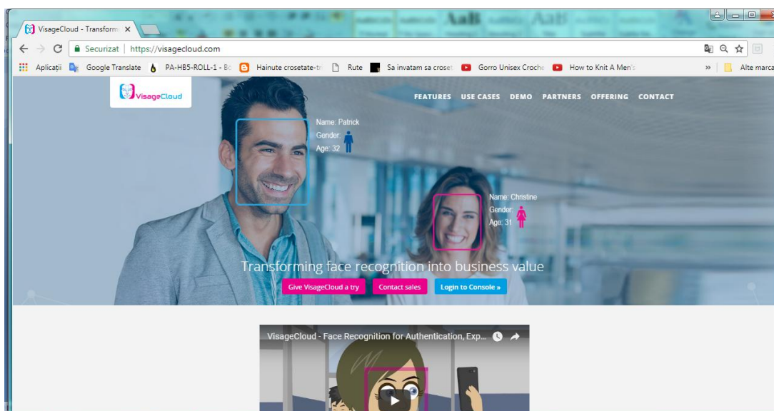
Fig. 40 VisageCloud Interface
